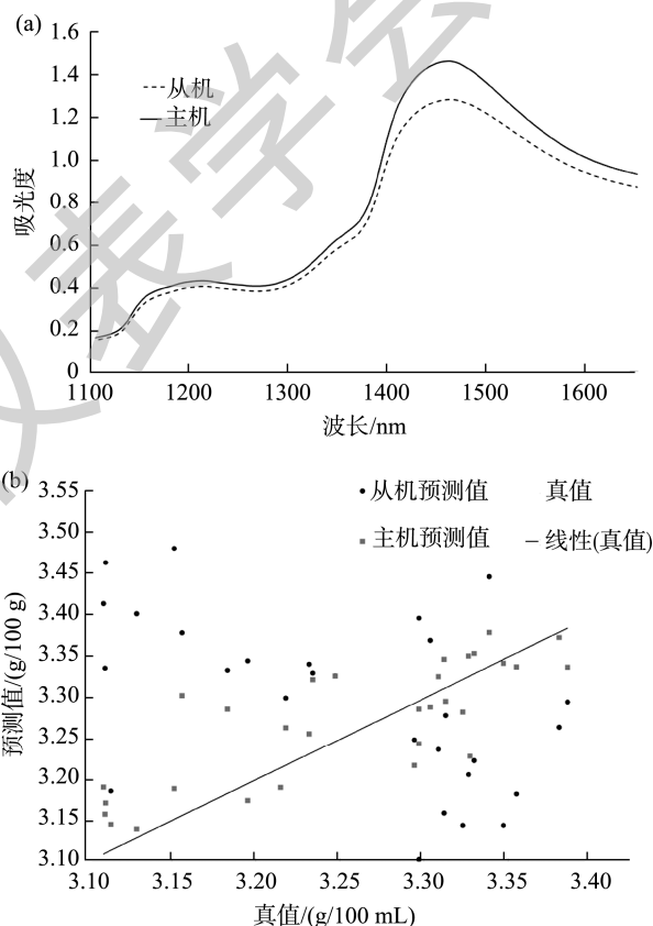
图1 不同近红外光谱仪检测结果对比(a)及光谱图预测结果(b) Fig.1 Comparison of detection results using different near-infrared spectrometers (a) and spectral prediction results (b)
